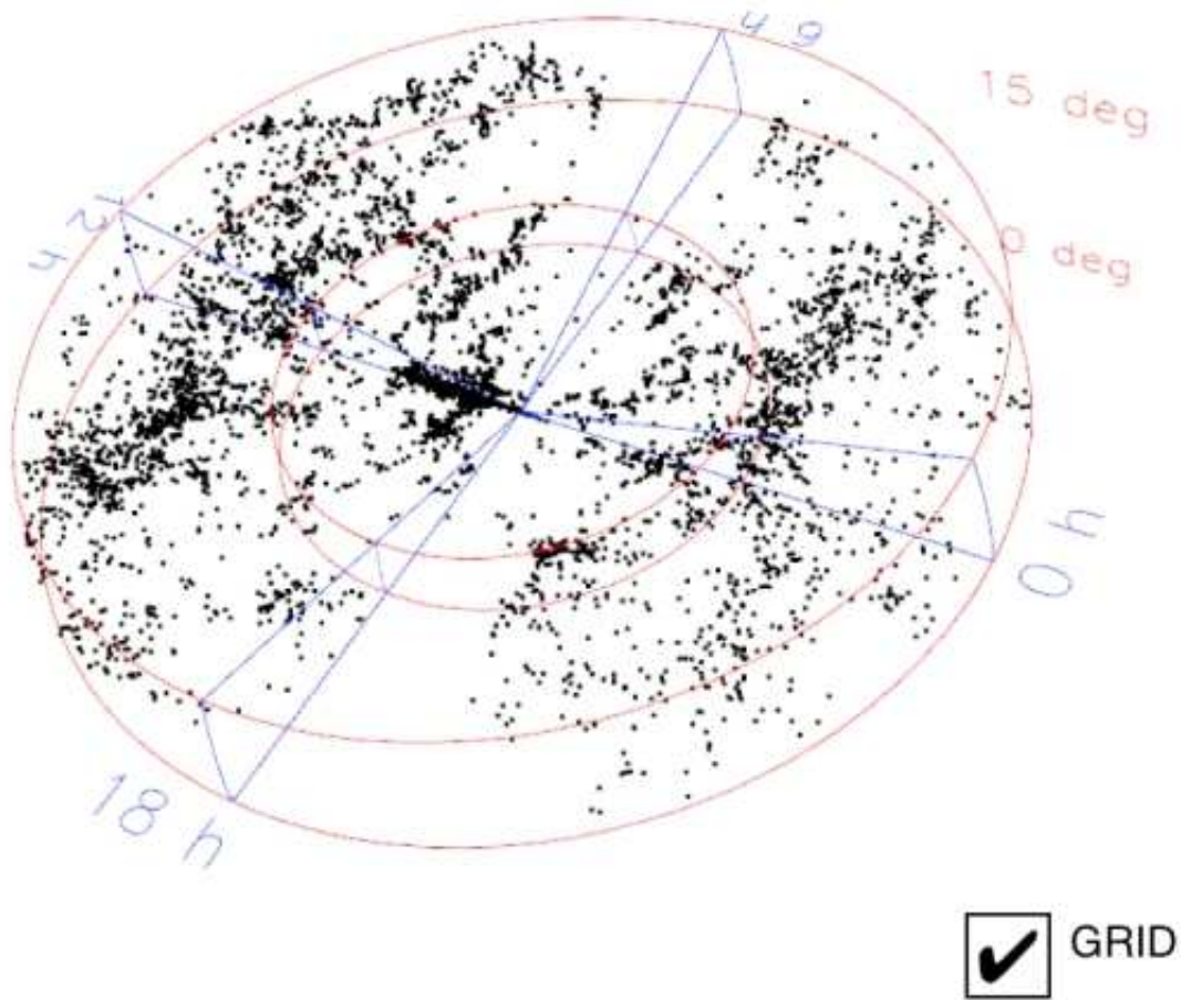
Figure 6. The large-scale structure of the Universe from the CfA2 galaxy survey. Plotted on this 3-d wedge diagram are galaxies between declination 0 and 15 degrees, and velocities below 10,000 km/s. There are gaps in the right ascension coverage between RA 5h30m to 6h30m, and 18h to 20h. The two sets of red declination rings indicate velocities 5,000 km/s and 10,000 km/s. Clicking the GRID button toggles the visibility of the coordinate lines. Click here for the interactive 3-d PDF of this figure.
