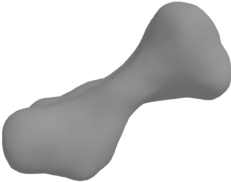
Figure 3. Asteroid 216 Kleopatra. The shape of this asteroid was determined using the S-band radar system of the Arecibo Observatory to create a series of delay Doppler images that are combined to determine the 3-d shape. See Ostro et al. (2000) for details. Click here for the interactive 3-d PDF of this figure.
