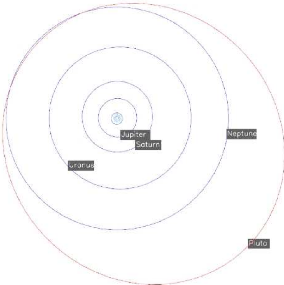
Figure 1. The inclination of Pluto's orbit (red) with respect to the plane of the Solar System is clearly apparent. The cyan line indicates Earth's orbit. Click here for the interactive 3-d PDF of this figure.
