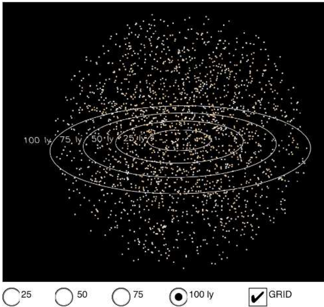
Figure 4. The 3-d location of stars within 100 light years of the Sun. Stellar distances are calculated using parallax data from the HIPPARCOS catalogue. Stars are colored according to spectral type. By clicking on one of the four buttons, stars within the indicated radius are displayed. The GRID button controls the visibility of the coordinate grid. Click here for the interactive 3-d PDF of this figure.
